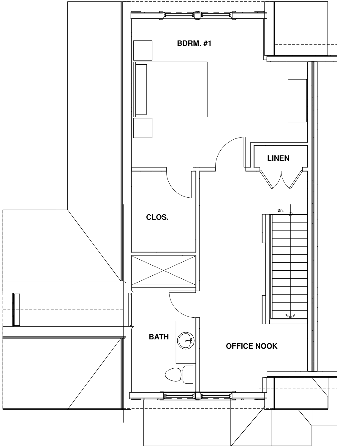
2ND FLOOR- UNIT TYPE 2
