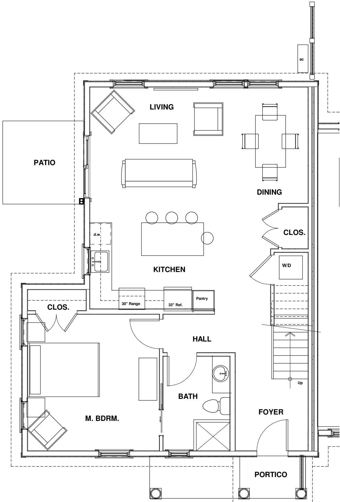
1ST FLOOR- UNIT TYPE 2
